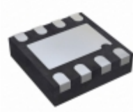
ADM7172ACPZ-1.3-R7 Analog Devices Inc. IC REG LDO 1.3V 2A 8-LFCSP
