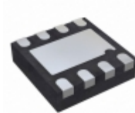
ADM7171ACPZ-2.5-R7 Analog Devices Inc. IC REG LDO 2.5V 1A 8-LFCSP
