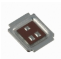
IRF6641TR1PBF Infineon Technologies MOSFET N-CH 200V 4.6A DIRECTFET
