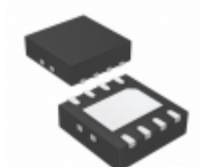
LTC2875HDD#PBF ADI (Analog Devices, Inc.) IC TXRX CAN 4MBPS 60V FP 8DFN
