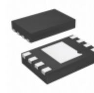
AT24CS02-MAHM-E Microchip Technology IC EEPROM 2KBIT 1MHZ 8UDFN
