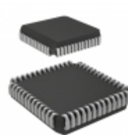
CY7C136-55JXIT Cypress Semiconductor Corp IC SRAM 16KBIT 55NS 52PLCC
