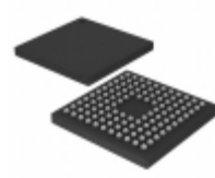
EFM32G890F128-BGA112T Silicon Labs IC MCU 32BIT 128KB FLASH 112BGA
