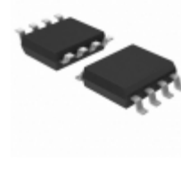
ISL6612CBZ Intersil IC DRVR MOSF SYNC BUCK OTP 8SOIC
