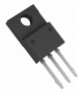
BA17807CP-E2 Rohm Semiconductor IC REG LDO 7V 1A TO-220CP
