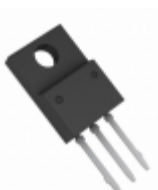
BA17806CP-E2 Rohm Semiconductor IC REG LDO 6V 1A TO-220CP
