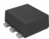
US6X5TR Rohm Semiconductor TRANS NPN 12V 2A TUMT6
