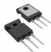
IRG7PH35UD1MPBF Infineon Technologies IGBT 1200V 50A 179W TO247AD
