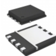
FDMS7698 Fairchild/ON Semiconductor MOSFET N-CH 30V 13.5A POWER56
