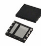
FDMS7700S Fairchild/ON Semiconductor MOSFET 2N-CH 30V 12A/22A POWER56
