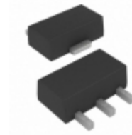
MCP1804T-2502I/MB Microchip Technology IC REG LDO 2.5V 0.1A SOT89-3
