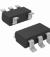
MCP1802T-5002I/OT Microchip Technology IC REG LDO 5V 0.3A SOT23-5
