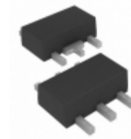
MCP1804T-2502I/MT Microchip Technology IC REG LDO 2.5V 0.1A SOT89-5
