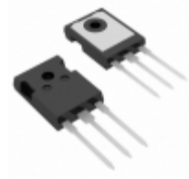
DSB80C45HB IXYS DIODE ARRAY SCHOTTKY 45V TO247AD
