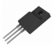
FDPF045N10A Fairchild/ON Semiconductor MOSFET N-CH 100V 67A TO-220-3
