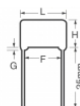
ECQ-P1H471JZ3 Panasonic Electronic Components CAP FILM 470PF 5% 50VDC RADIAL
