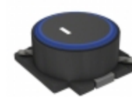
SLF12565T-4R2N5R5-PF TDK Corporation FIXED IND 4.2UH 5.5A 15 MOHM SMD
