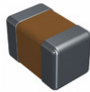
CDR31BX102BKWRAC Electro-Films (EFI) / Vishay CAP CER 1000PF 100V BX 0805
