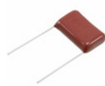
ECQ-E6394KFW Panasonic Electronic Components CAP FILM 0.39UF 10% 630VDC RAD
