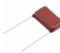
ECQ-E6394KFA Panasonic Electronic Components CAP FILM 0.39UF 10% 630VDC RAD
