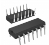
MCP4922-E/P Microchip Technology IC DAC 12BIT DUAL W/SPI 14DIP
