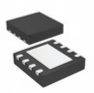
MCP4921T-E/MC Microchip Technology DAC 12BIT SGL SPI 8DFN
