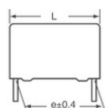
B32923C3564K EPCOS (TDK) CAP FILM 0.56UF 10% 305VAC RAD
