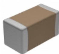
CDR32BP241BJZRAT Electro-Films (EFI) / Vishay CAP CER 240PF 100V 5% BP 1206
