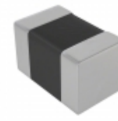
C0805C393K4JAC7800 KEMET CAP CER 0.039UF 16V U2J 0805
