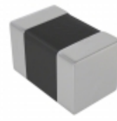
C0805C393K4RACTU KEMET CAP CER 0.039UF 16V X7R 0805
