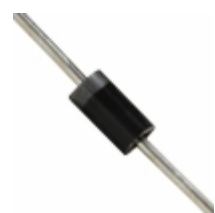
BZX85C12_T50R Fairchild/ON Semiconductor DIODE ZENER 12V 1W DO41
