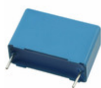
B32523Q1106K189 EPCOS (TDK) CAP FILM 10UF 10% 100VDC RADIAL
