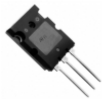
HD1760JL STMicroelectronics TRANS NPN 800V 36A TO-264
