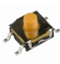
KSC411G 70 SH C&K SWITCH TACTILE SPST-NO 0.05A 32V
