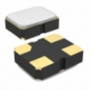
SG-310SCN 66.6660MM0 Epson OSC XO 66.666MHZ CMOS SMD
