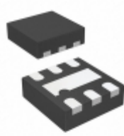
MIC5367-1.5YMT-TR Microchip Technology IC REG LDO 1.5V 0.15A 6TMLF
