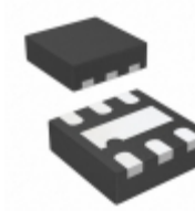
MIC5368-1.5YMT-TR Microchip Technology IC REG LDO 1.5V 0.15A 6TMLF
