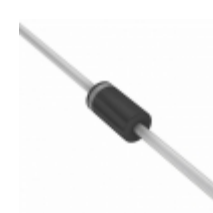
1N4759A-TR Vishay Semiconductor Diodes Division DIODE ZENER 62V 1.3W DO41
