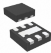
NCP121AMX185TCG ON Semiconductor IC REG LDO 1.85V 0.15A 6XDFN
