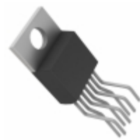
LT3091HT7#PBF ADI (Analog Devices, Inc.) IC REG LIN NEG ADJ 1.5A TO220-7
