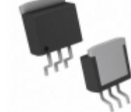
MCP1826S-3002E/EB Microchip Technology IC REG LDO 3V 1A 3DDPAK
