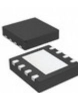
MCP4152T-502E/MF Microchip Technology IC POT DGTL SNGL 5K RHEO 8DFN
