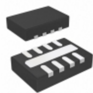
LT3470HDDDB#TRPBF Linear Technology IC REG BUCK ADJ 0.2A 8DFN
