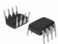
NCP1002PG ON Semiconductor IC OFFLINE SWIT PWM UVLO HV 8DIP
