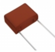
ECW-F2W824JA Panasonic Electronic Components CAP FILM 0.82UF 5% 450VDC RADIAL
