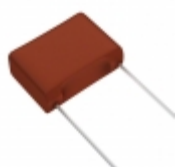
ECW-F2W684JA Panasonic Electronic Components CAP FILM 0.68UF 5% 450VDC RADIAL
