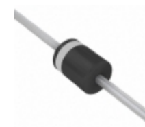
SUF30J-E3/73 Vishay Semiconductor Diodes Division DIODE GEN PURP 600V 3A P600
