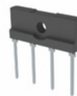
TS10KL100 D3G TSC (Taiwan Semiconductor) BRIDGE RECT 1PHASE 1KV 10A KBJL
