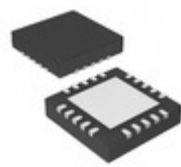
MCP23008T-E/ML Microchip Technology IC I/O EXPANDER I2C 8B 20QFN
