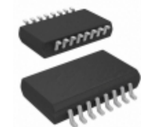
AD7543GKR Analog Devices Inc. IC DAC 12BIT SRL INP MULT 16SOIC
