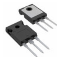
IRG7PH37K10DPBF Infineon Technologies IGBT 1200V 45A 216W TO247AC
