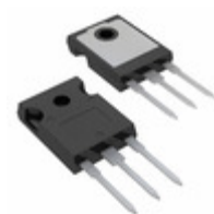
IRG7PH35UPBF Infineon Technologies IGBT 1200V 55A 210W TO247AC
