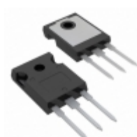
IRG7PH42UD-EP Infineon Technologies IGBT 1200V 85A 320W TO247AD
