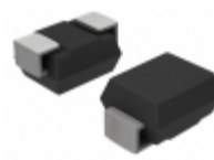
NP0900SBT3G ON Semiconductor THYRISTOR 75V 80A SMB
