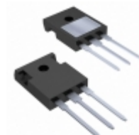
IXTJ6N150 IXYS MOSFET N-CH 1500V 3A ISOTO-247
