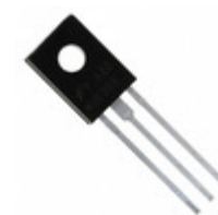
BD3756STU Fairchild/ON Semiconductor TRANS NPN 45V 2A TO-126
