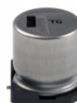
EEV-TG1C102UQ Panasonic Electronic Components CAP ALUM 1000UF 20% 16V SMD
