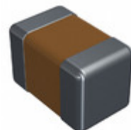
CDR31BP100BJUMAB Electro-Films (EFI) / Vishay CAP CER 10PF 100V BP 0805
