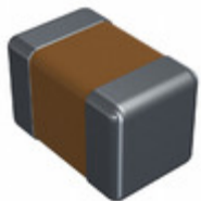
CDR31BP100BJMSAB Electro-Films (EFI) / Vishay CAP CER 10PF 100V BP 0805
