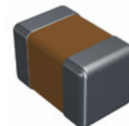
CDR31BP100BJMRAR Electro-Films (EFI) / Vishay CAP CER 10PF 100V BP 0805
