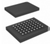
SST39WF1602-70-4C-B3KE Micrel / Microchip Technology IC FLASH 16MBIT 70NS 48TFBGA
