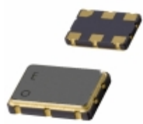
EG-2121CA 125.0000M-VGRNL3 EPSON OSC SO 125.000MHZ LVDS SMD
