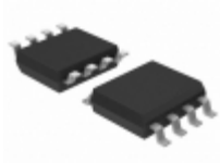
ACS715ELCTR-20A-T Allegro MicroSystems, LLC SENSOR CURRENT HALL 20A DC
