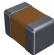
CDR31BP180BFWMAT Electro-Films (EFI) / Vishay CAP CER 18PF 100V BP 0805
